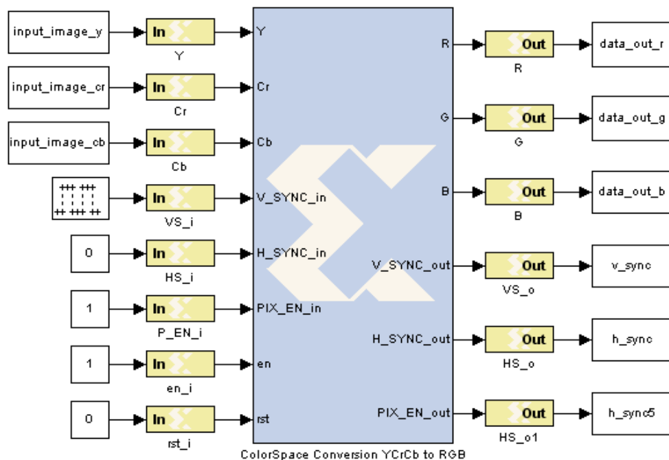
Figure 9: System Generator Testbench
