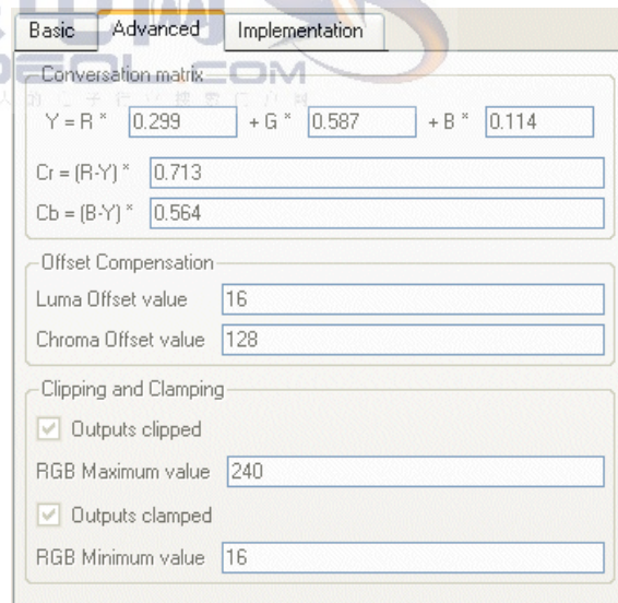
Figure 7: Advanced Tab
